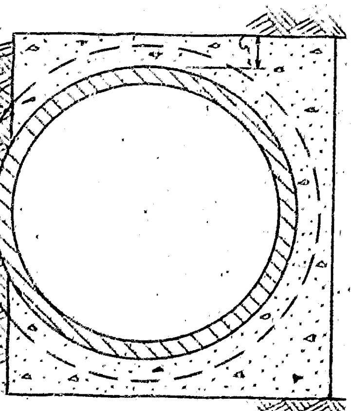
BENEATH ROADWAYS PIPE ENCASUREMENT
